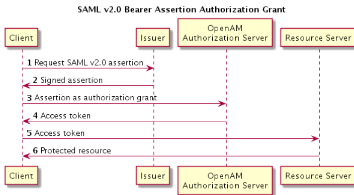
Figure 13.10. SAML v2.0 Bearer Assertion Authorization Grant
