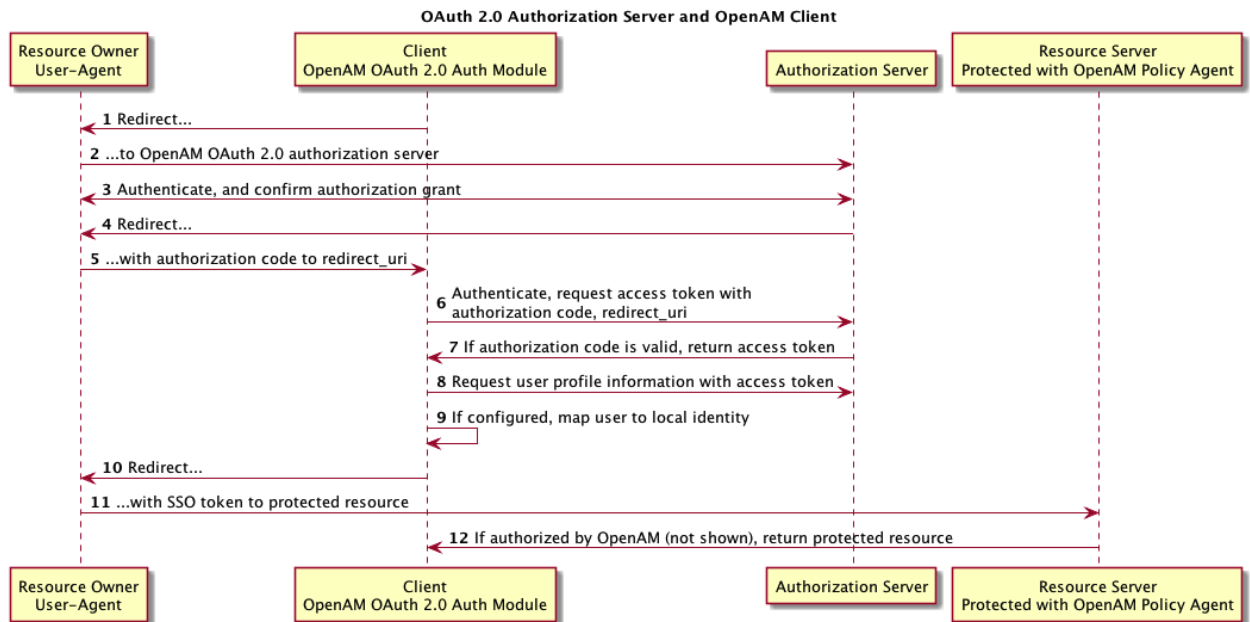
Figure 13.11. OpenAM as OAuth 2.0 Client and Authorization Server
