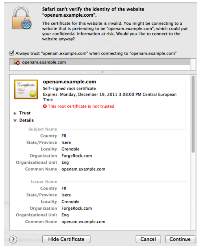
Figure 23.1. Unknown Certificate
