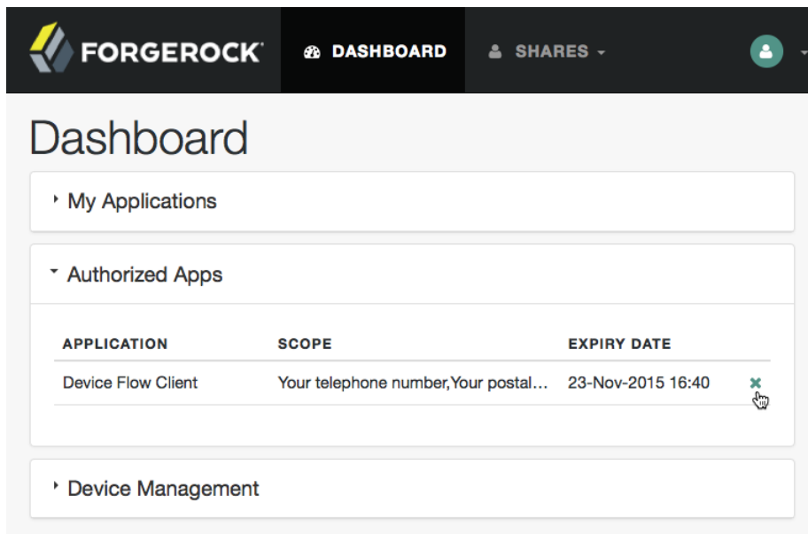
Figure 13.16. OAuth 2.0 Self-Service
