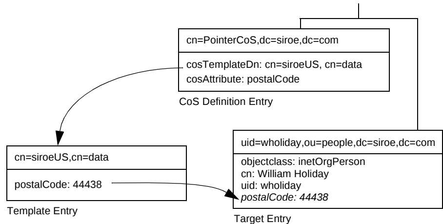
Figure 5-1 Example of a Pointer CoS Definition and Template
