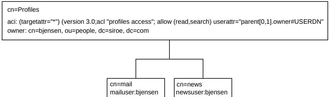
Figure 6-1 Using Inheritance With the userattr Keyword
