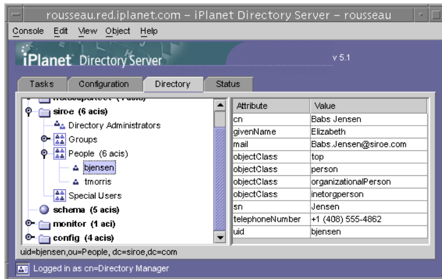
Figure 1-4 Directory Tab of the Directory Server Console
