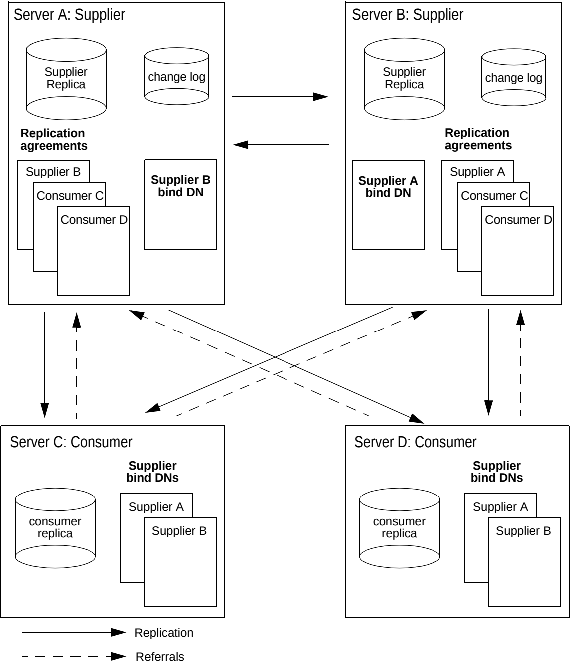
Figure 8-3 Detailed view of Multi-Master Replication
