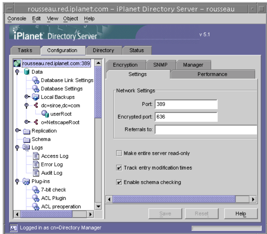
Figure 1-3 Configuration Tab of the Directory Server Console
