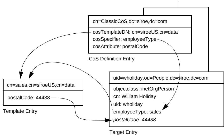
Figure 5-3 Example of a Classic CoS Definition and Template
