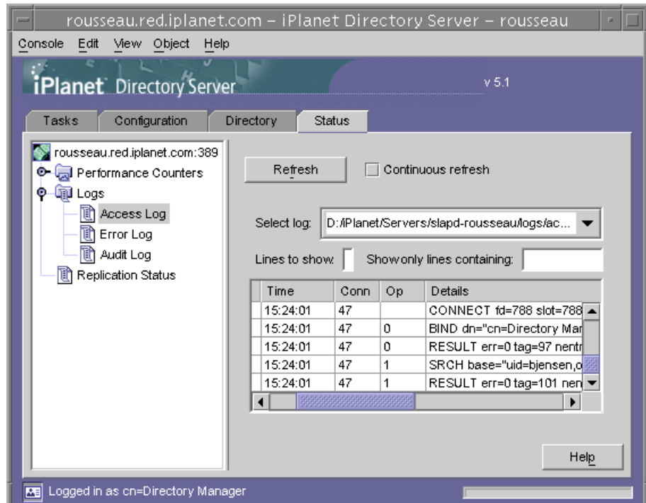
Figure 1-5 Status Tab of the Directory Server Console
