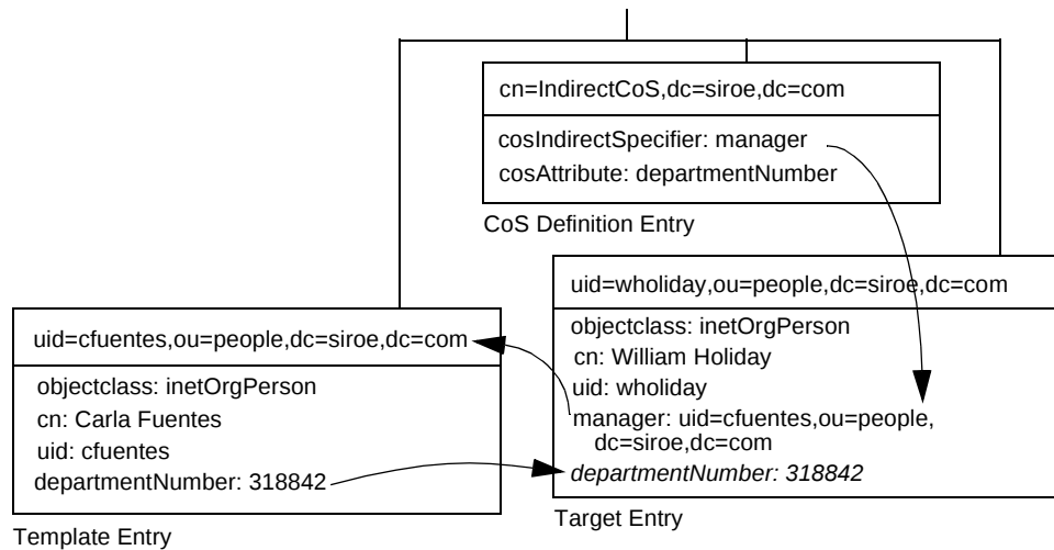
Figure 5-2 Example of an Indirect CoS Definition and Template
