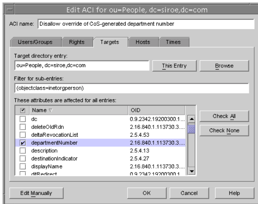
Figure 6-3 The Access Control Editor Dialog
