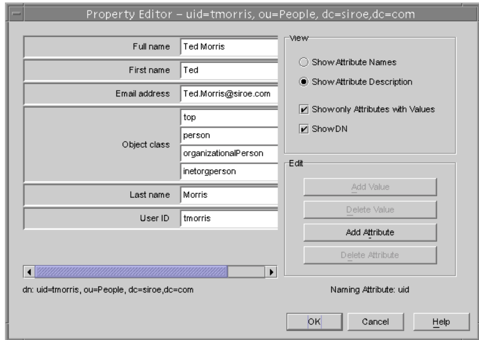
Figure 2-1 iPlanet Directory Server Console - Property Editor
